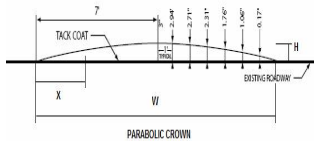
Figure 1. Speed Hump Profile
